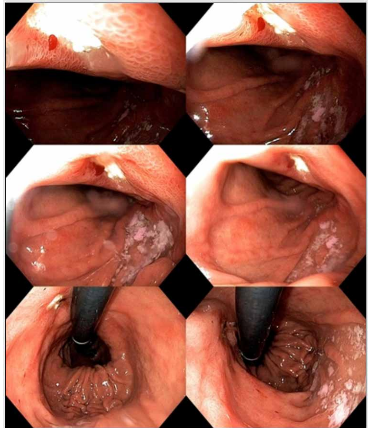
Collage:Cameron ulcer
